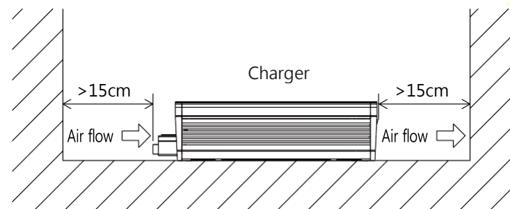
Figure 3-1 set-up recommendation
