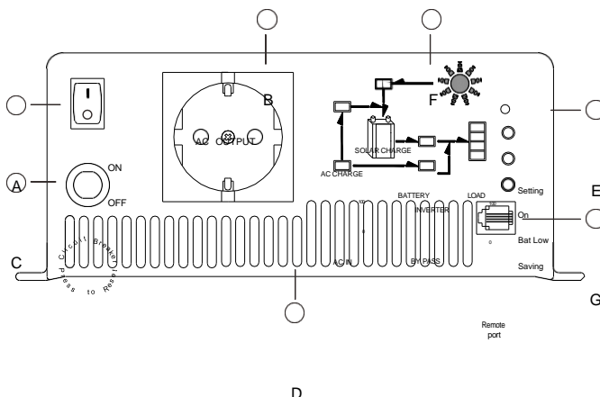
Figure 3.1: Front Panel (TN-1500)
