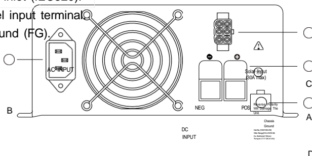
Fig 3.2: Rear Panel (TN-1500)
