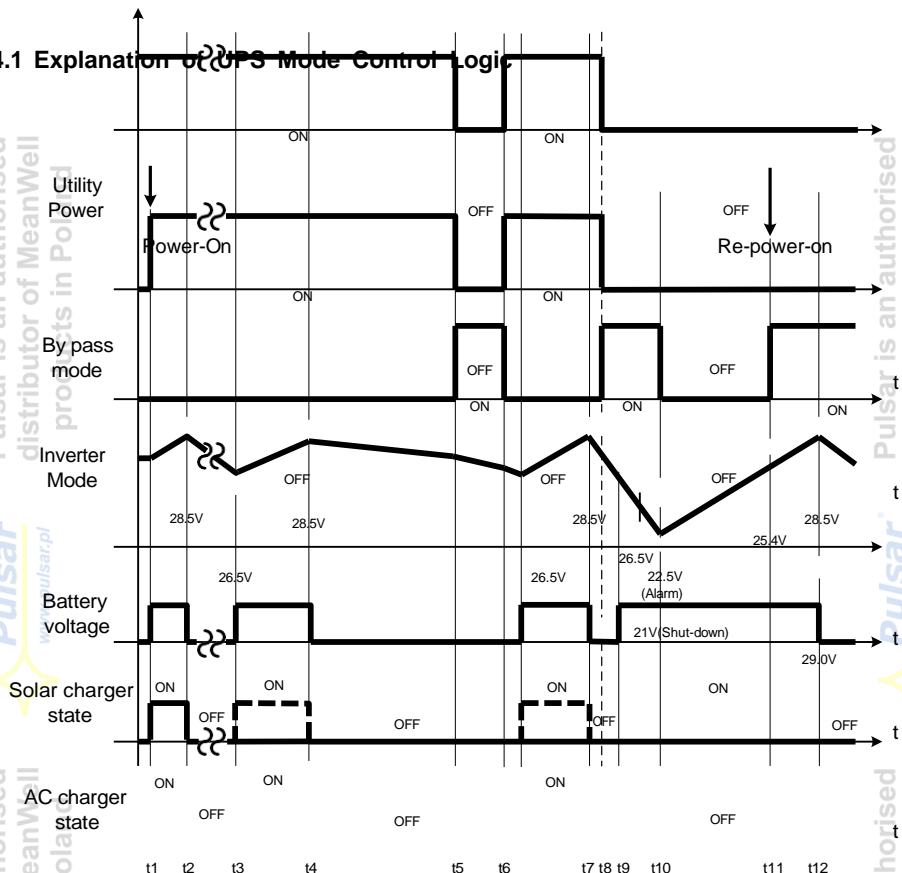
Figure 4.1: Diagram of UPS Mode Control Logic
