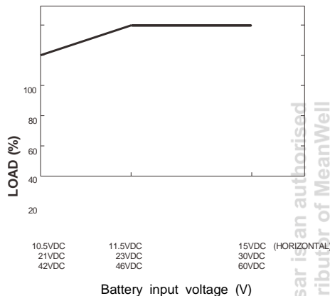
Figure 7.3 Input derating curve
