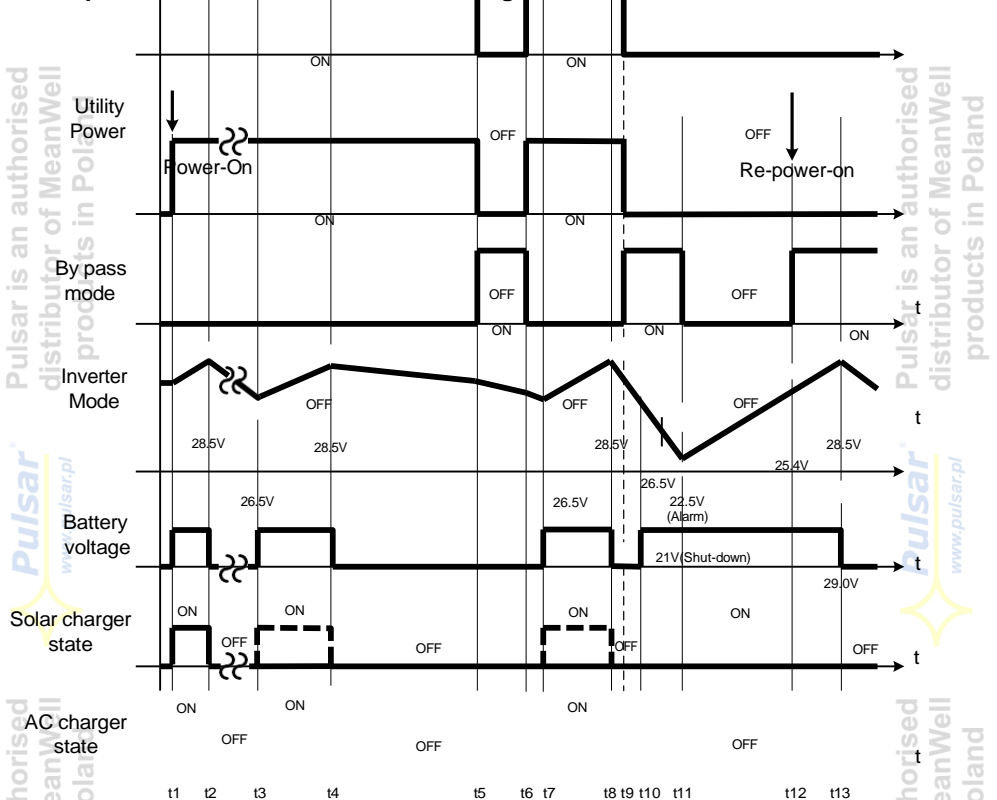
Figure 4.1 Diagram of UPS mode control logic
