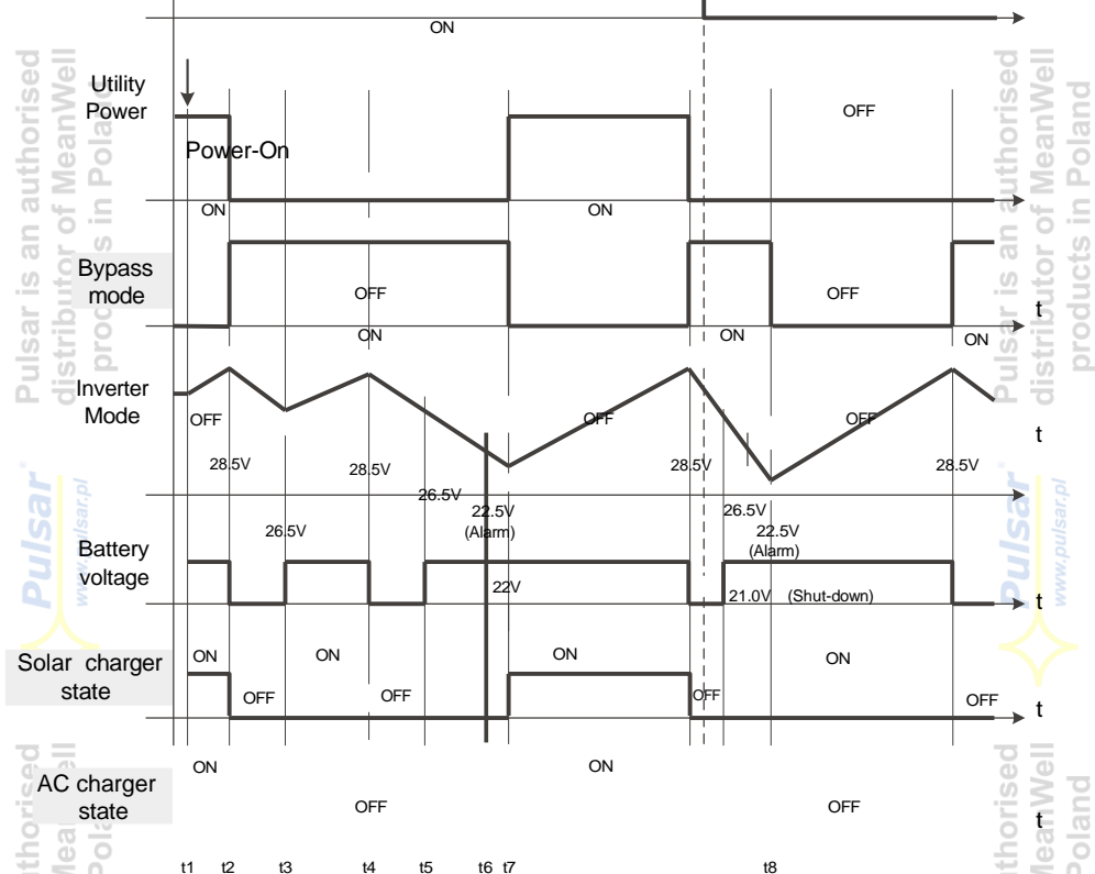
Figure 4.2 Diagram of energy saving mode control logic
