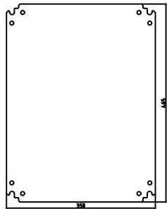
Mounting plate
