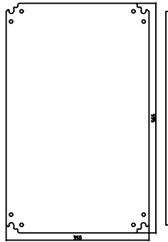
Mounting plate
