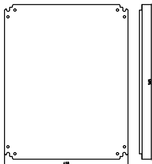
Mounting plate
