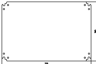
Mounting plate
