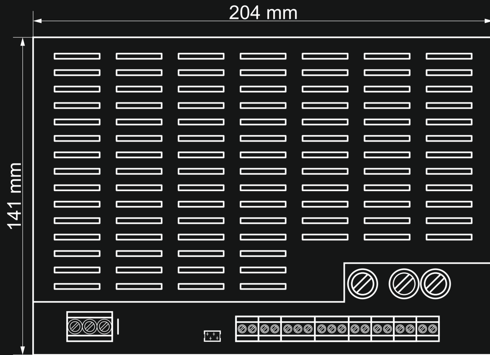
Front
