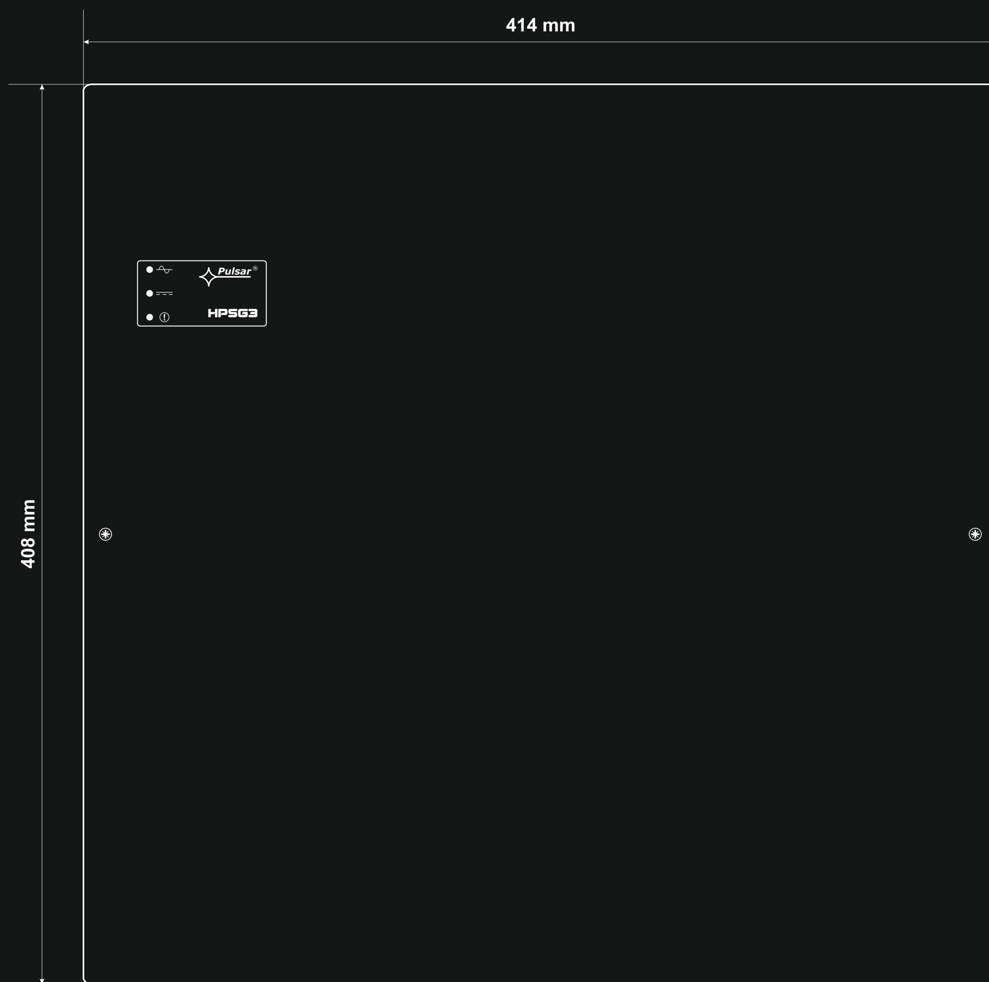
Front
