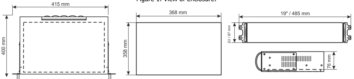
Figure 2. Dimensions.
