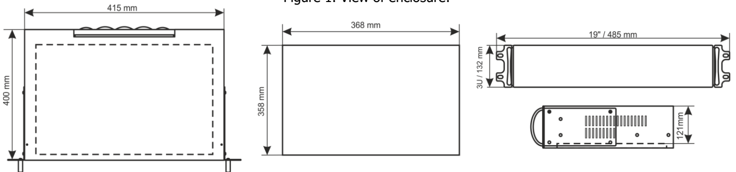
Figure 2. Dimensions.
