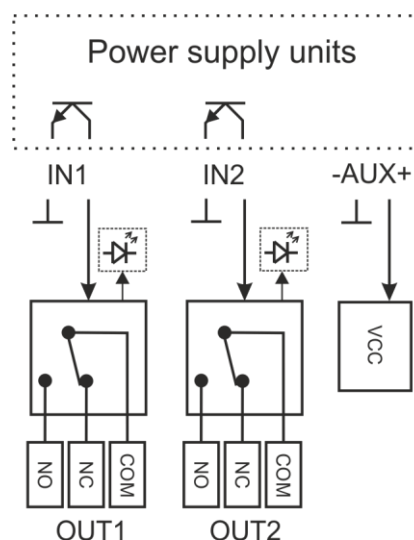
Fig. 2. Block diagram.
