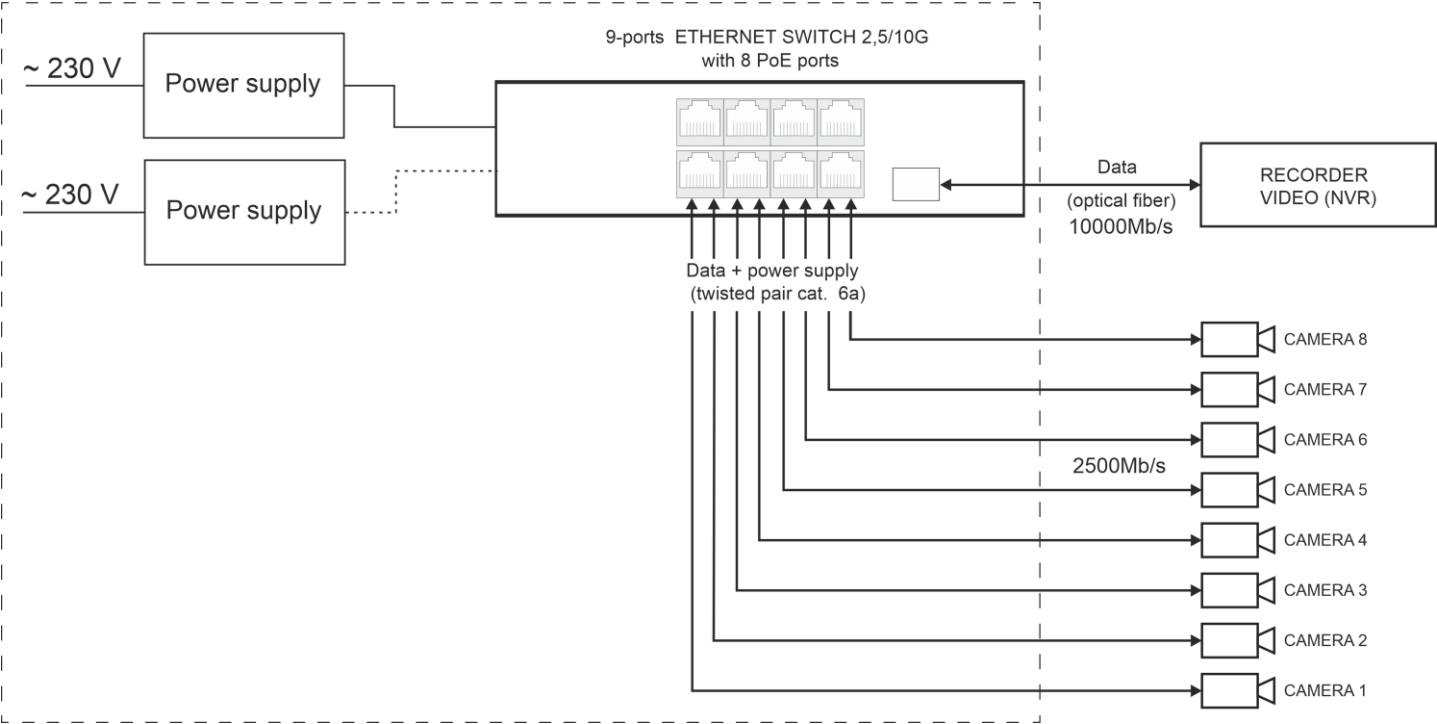
Fig. 1. Block diagram.
