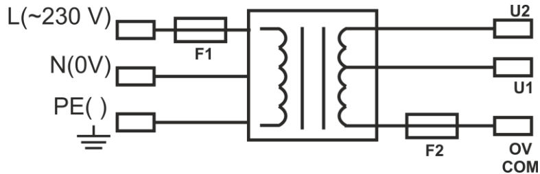
Fig.1. Block diagram of the PSU.
