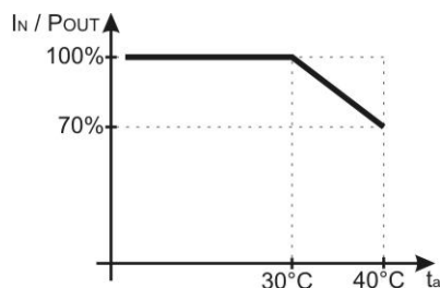
Graph 1. Relation between output current and ambient
