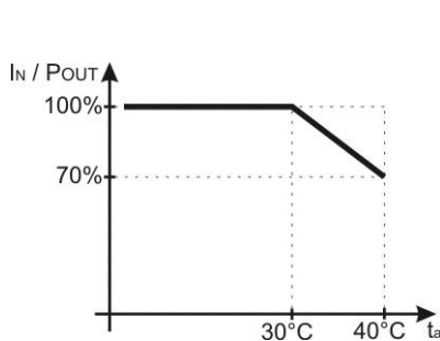
Graph 1. Relation between output current and ambient temperature (instantaneous load).
