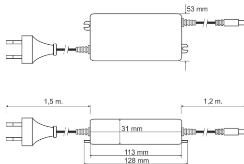
Fig.1. Dimension of power supply.
