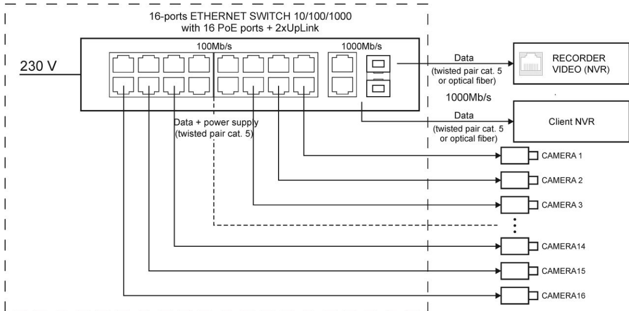
Fig. 1. Block diagram.
