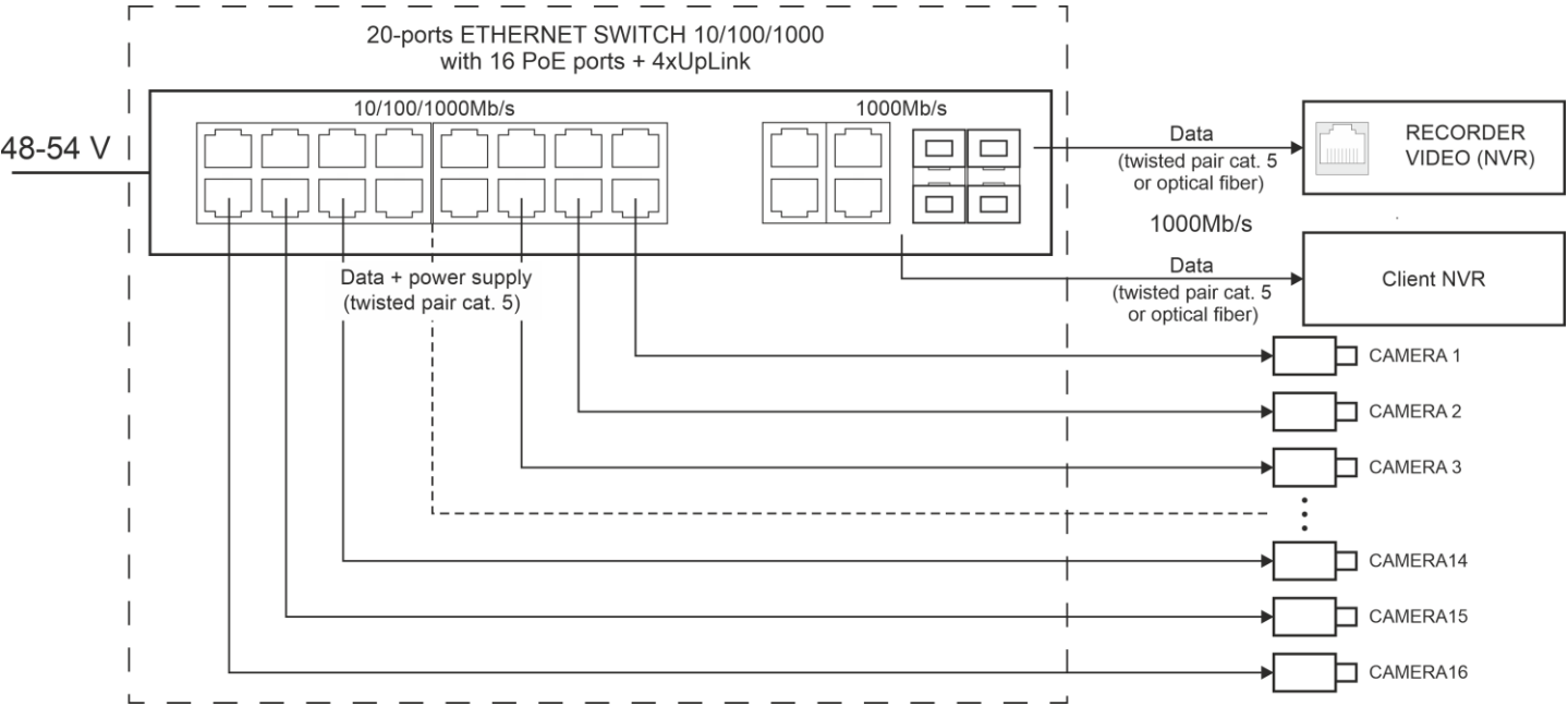
Fig. 1. Block diagram.
