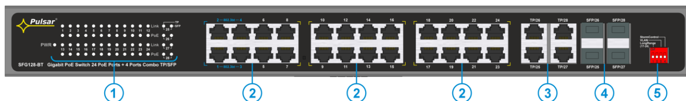
Fig. 2. Front panel.
