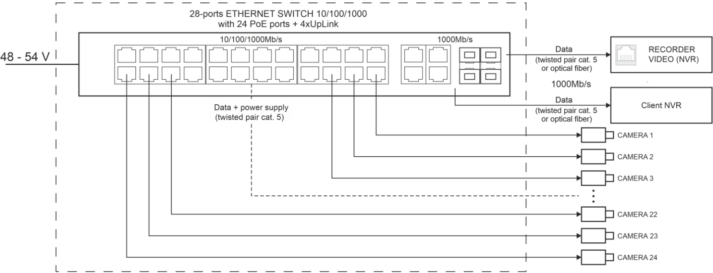
Fig. 1. Block diagram.
