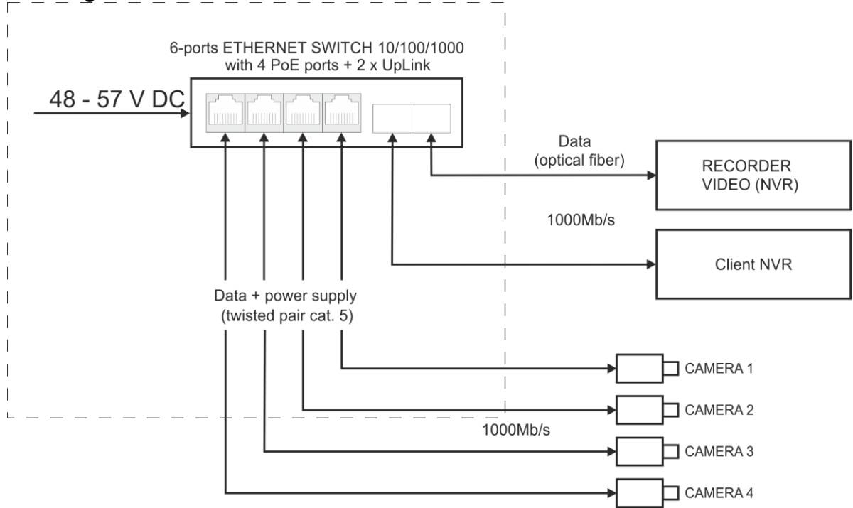
Fig. 1. Block diagram.
