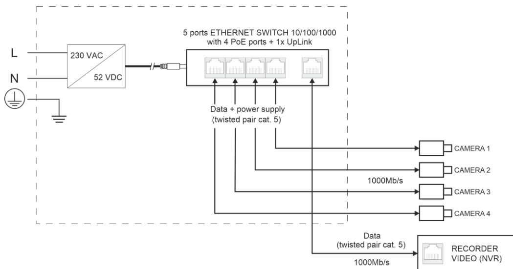
Fig. 1. Block diagram.
