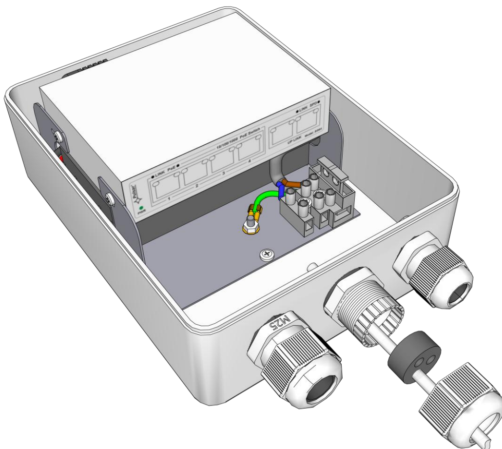
Fig.4. Example of installation.
