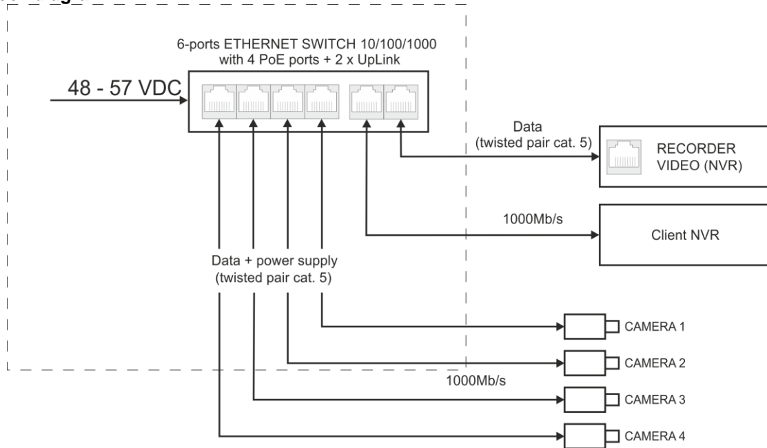
Fig. 1. Block diagram.
