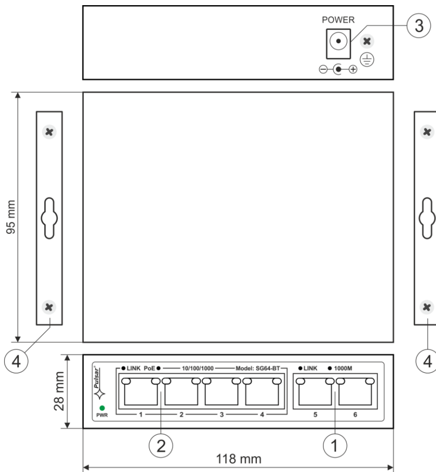
Fig. 2. View of the switch.
