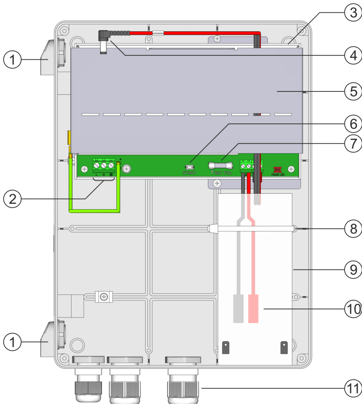
Fig. 2. View of PSU.
