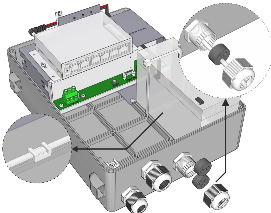
Fig. 3. Example of installation
