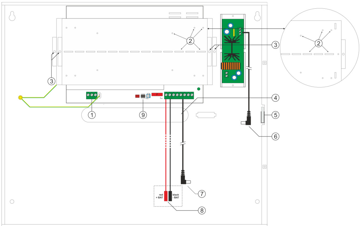
Fig.3. View of device.
