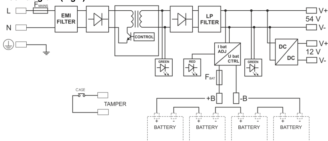
Fig.1. Block diagram of PSU.
