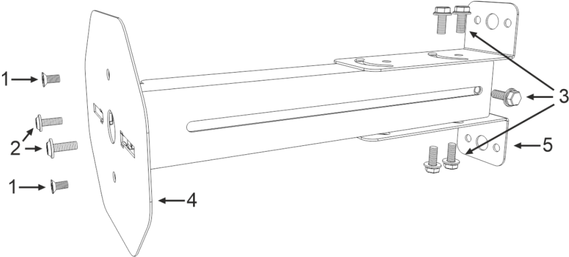
Fig.2. Installing the handle
