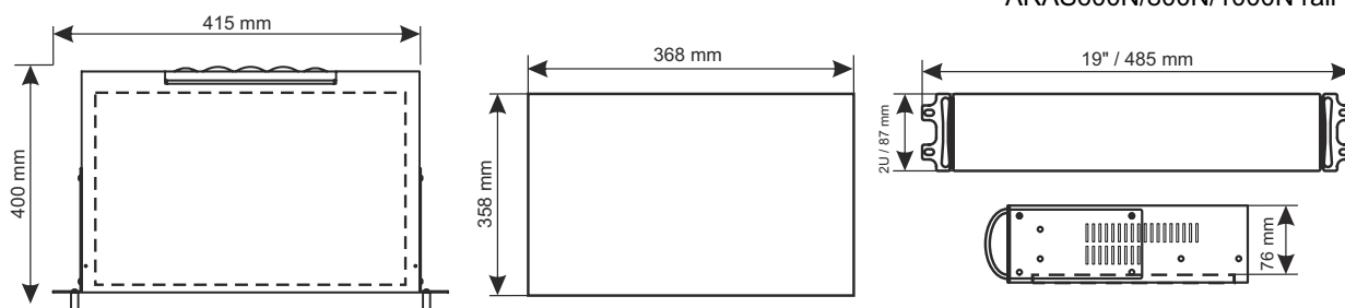
Mounting on a ARAS600N/800N/1000N rail
