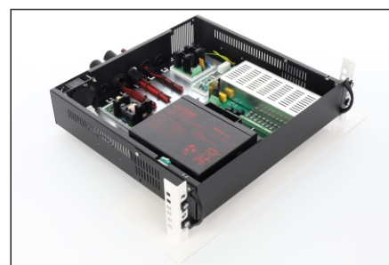
Front mounting
