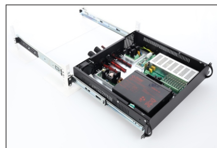
Mounting on a ARAS600N/800N/1000N rail
