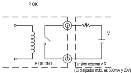
Fig. 4.2 Circuito interno de P OK (Relé, total 10W)
