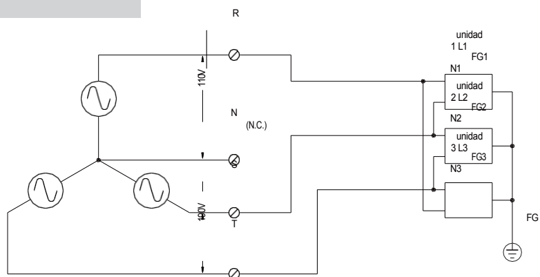
FIG. C: SISTEMA 3 \psi 4W 190/110VAC
